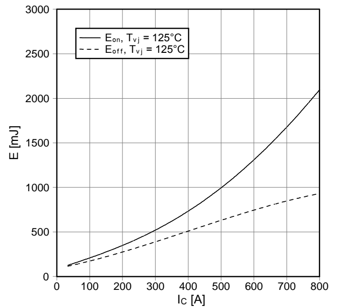
Schaltverluste IGBT-Wechselr. (typisch) switching losses IGBT-inverter (typical) E_{on} = f(I_C) , E_{off} = f(I_C) V_{GE} = \pm 15\text{ V} , R_{Gon} = 2,7\ \Omega , R_{Goff} = 3,6\ \Omega , V_{CE} = 1800\text{ V} , C_{GE} = 68\text{ nF}
