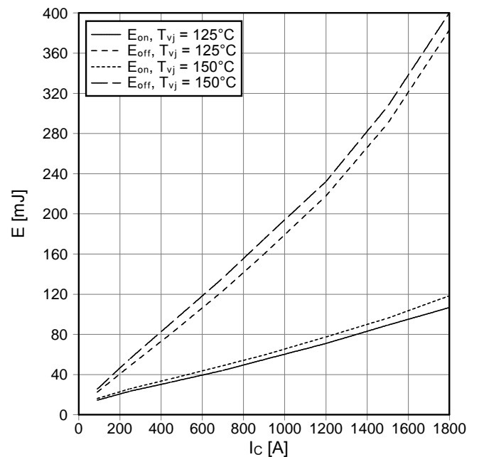
Schaltverluste IGBT-Wechselr. (typisch) switching losses IGBT-inverter (typical) E_{on} = f(I_C) , E_{off} = f(I_C) V_{GE} = \pm 15\text{ V} , R_{Gon} = 1.5\ \Omega , R_{Goff} = 0.9\ \Omega , V_{CE} = 600\text{ V}
