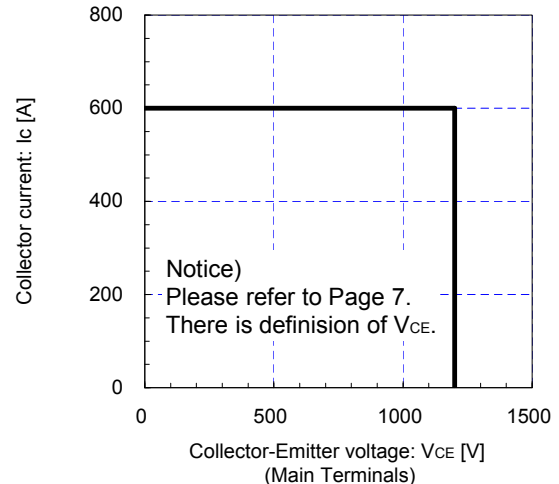
Reverse bias safe operating area (max.) +V_{ge}=15V, -V_{ge}\le 15V, R_g\ge 0.93\Omega, T_j=150^\circ C
