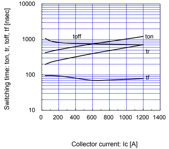
Switching time vs. Collector current (typ.) V_{CC}=300V, V_{GE}=\pm 15V, R_G=2.2\Omega, T_j=150^\circ C
