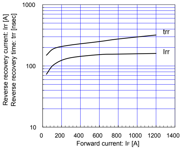
Reverse Recovery Characteristics (typ.) Vcc=300V, VGE=±15V, RG=2.2Ω, Tj=150°C
