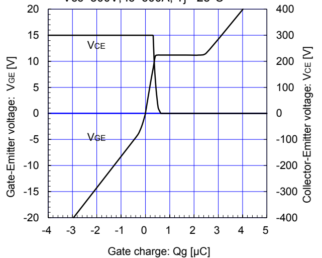
Dynamic Gate Charge (typ.) V CC = 300V, I C = 600A, T j = 25°C
