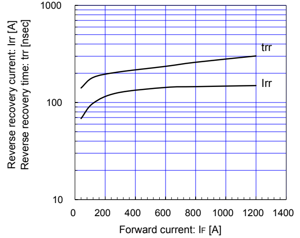
Reverse Recovery Characteristics (typ.) Vcc=300V, VGE=±15V, RG=2.2Ω, Tj=125°C
