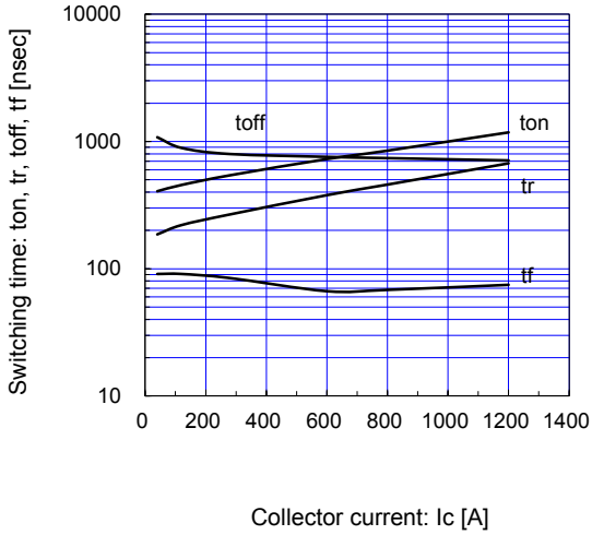
Switching time vs. Collector current (typ.) V_{CC}=300V, V_{GE}=\pm 15V, R_G=2.2\Omega, T_j=125^\circ C
