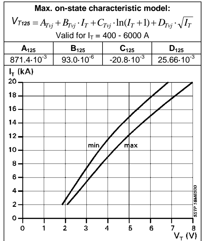
Fig. 3 On-state voltage characteristics, T_{vj\_start} = 125 \text{ }^\circ\text{C} , 10 ms sine half wave
